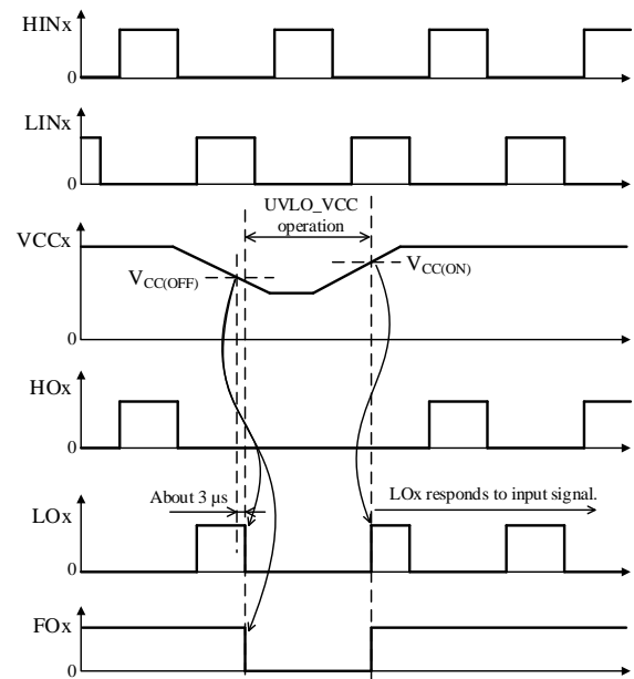
Figure 12-14. Operational Waveforms of UVLO_VCC
