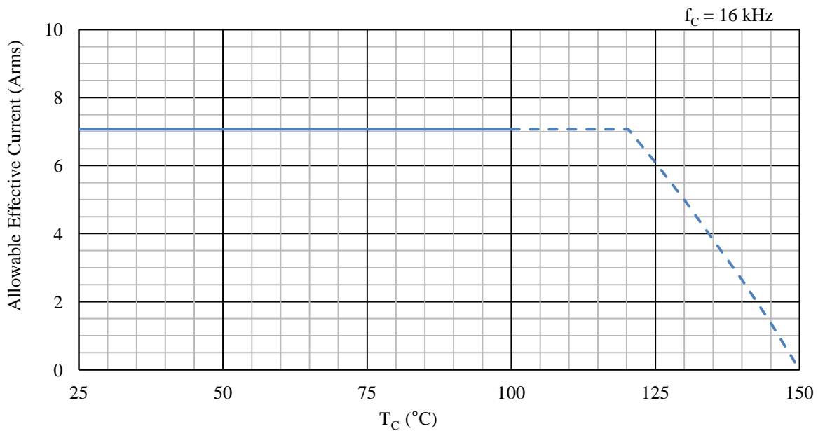
Figure 15-69. Allowable Effective Current, 10 A Device ( f_c = 16\text{ kHz} )
