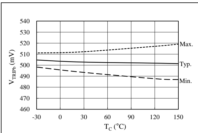
Figure 15-24. Overcurrent Protection Threshold Voltage, V_{TRIP} vs. T_C
