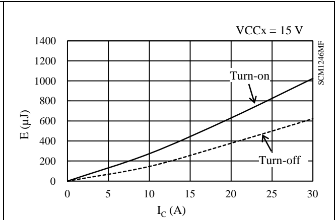
Figure 15-65. Low-side Switching Loss (T j = 25 °C)
