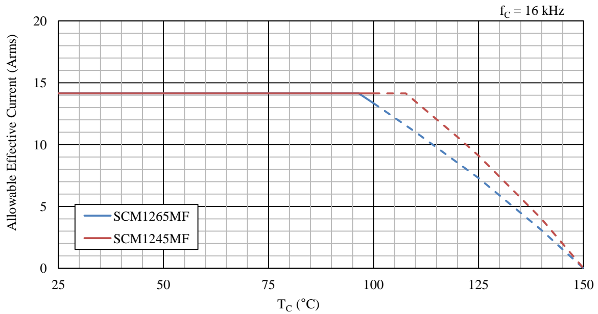
Figure 15-73. Allowable Effective Current, 20 A Device ( f_c = 16 \text{ kHz} )
