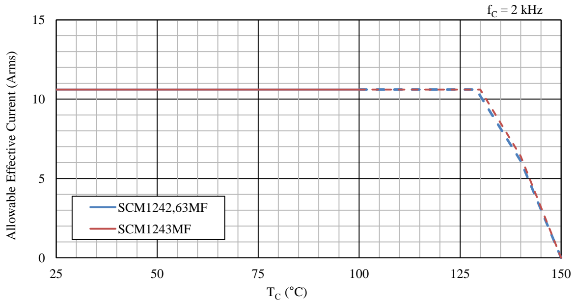
Figure 15-70. Allowable Effective Current, 15 A Device ( f_c = 2 kHz)
