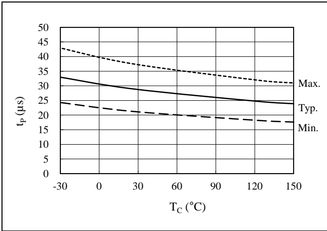
Figure 15-26. Overcurrent Protection Hold Time, t_p vs. T_C
