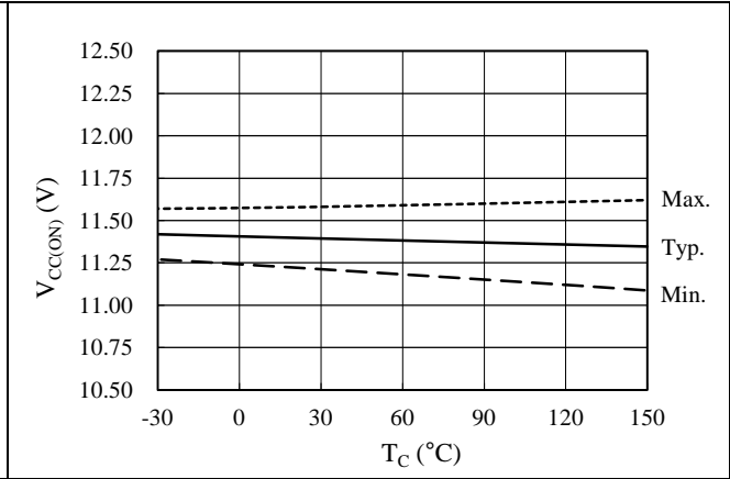
Figure 15-9. Logic Operation Start Voltage, V_{CC(ON)} vs. T_C
