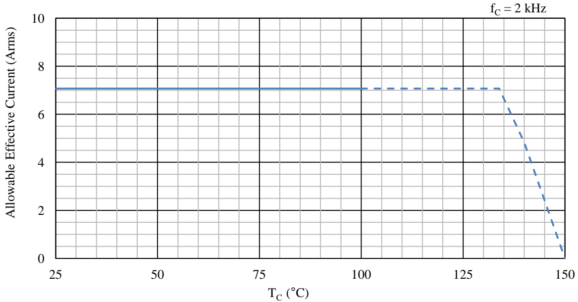
Figure 15-68. Allowable Effective Current, 10 A Device ( f_c = 2\text{ kHz} )
