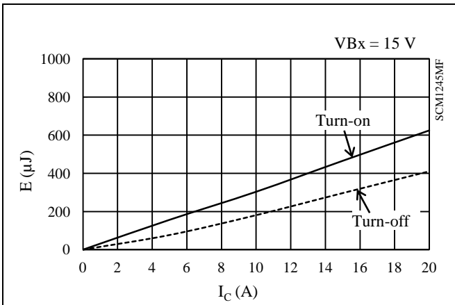
Figure 15-58. High-side Switching Loss ( T_j = 125\text{ }^\circ\text{C} )
