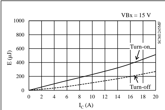
Figure 15-56. High-side Switching Loss ( T_j = 25\text{ }^\circ\text{C} )
