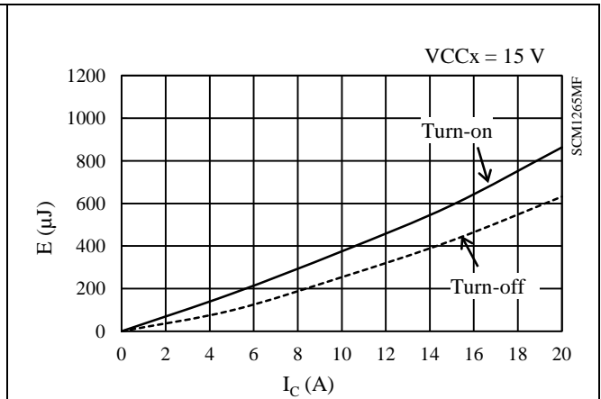
Figure 15-53. Low-side Switching Loss ( T_j = 25\text{ }^\circ\text{C} )
