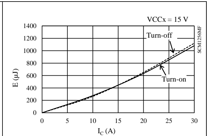
Figure 15-61. Low-side Switching Loss ( T_j = 25\text{ }^\circ\text{C} )
