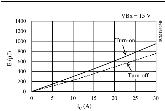
Figure 15-66. High-side Switching Loss (T j = 125 °C)
