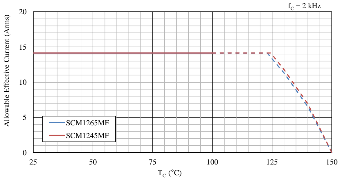
Figure 15-72. Allowable Effective Current, 20 A Device ( f_c = 2 \text{ kHz} )
