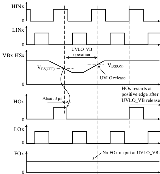
Figure 12-13. Operational Waveforms of UVLO_VB
