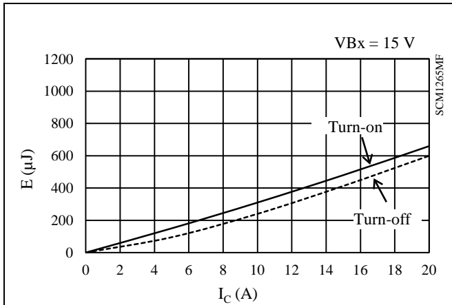
Figure 15-52 High-side Switching Loss ( T_j = 25\text{ }^\circ\text{C} )
