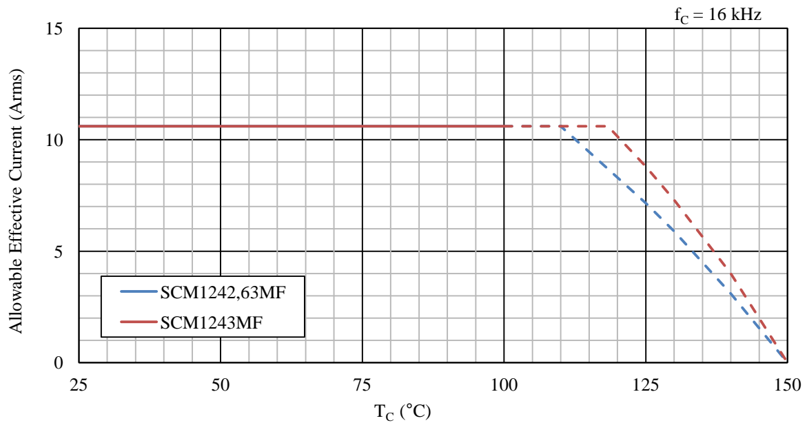
Figure 15-71. Allowable Effective Current, 15 A Device ( f_c = 16 kHz)
