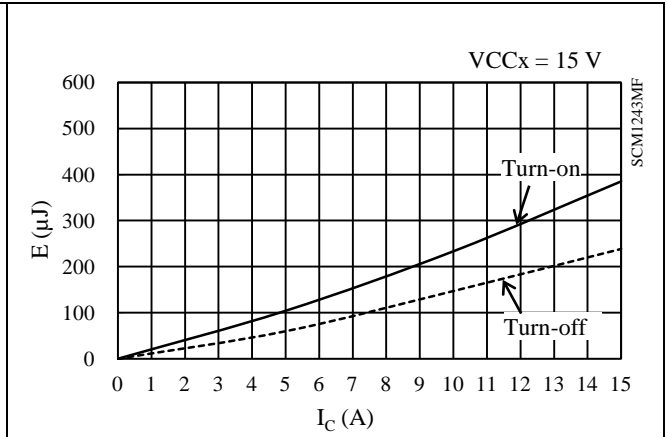
Figure 15-49. Low-side Switching Loss (T j = 25 °C)
