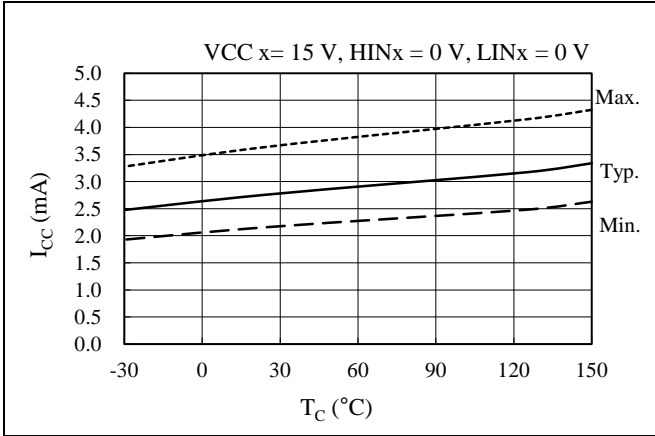
Figure 15-2. Logic Supply Current in 3-phase Operation, I_{CC} vs. T_C
