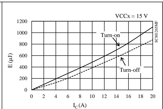
Figure 15-55. Low-side Switching Loss ( T_j = 125\text{ }^\circ\text{C} )
