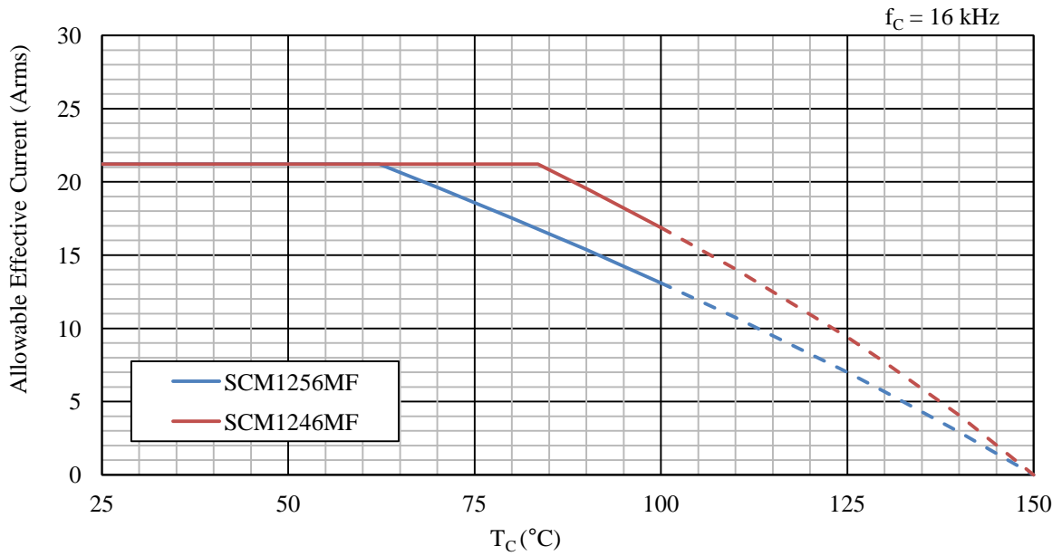
Figure 15-75. Allowable Effective Current, 30 A Device ( f_c = 16 kHz)
