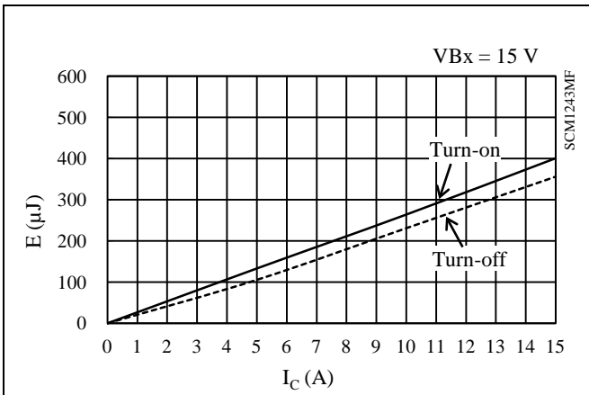
Figure 15-50. High-side Switching Loss (T j = 125 °C)
