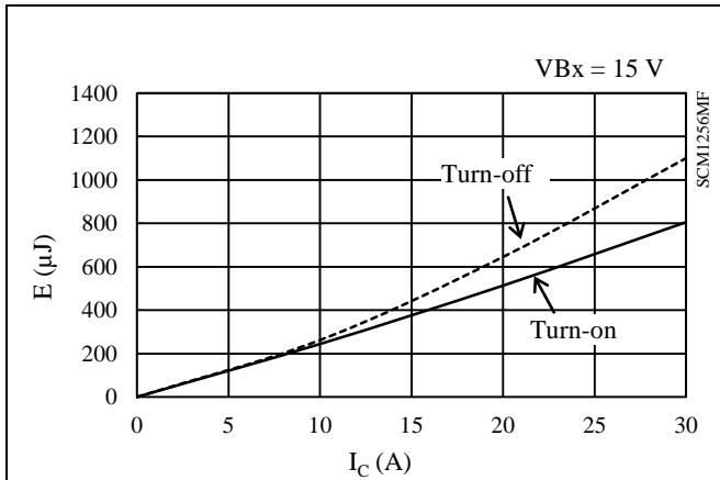
Figure 15-60. High-side Switching Loss ( T_j = 25\text{ }^\circ\text{C} )
