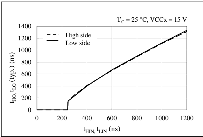
Figure 15-22. Typical Output Pulse Widths, t_{HO} , t_{LO} vs. Input Pulse Widths, t_{HIN} , t_{LIN}
