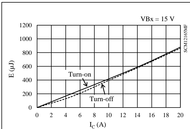
Figure 15-54. High-side Switching Loss ( T_j = 125\text{ }^\circ\text{C} )
