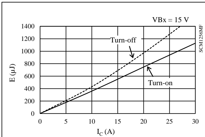
Figure 15-62. High-side Switching Loss ( T_j = 125\text{ }^\circ\text{C} )
