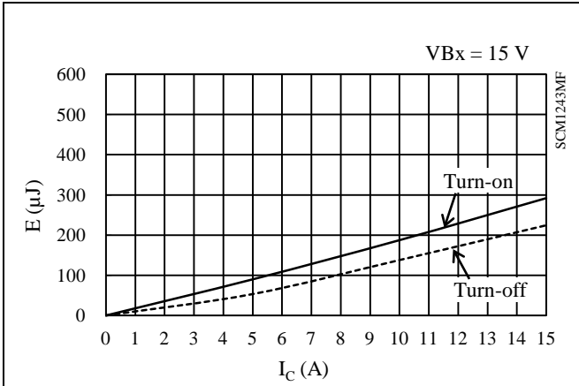
Figure 15-48 High-side Switching Loss (T j = 25 °C)
