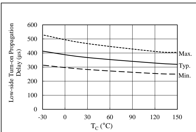
Figure 15-18. Low-side Turn-on Propagation Delay vs. T C (from LIN x to LO x )
