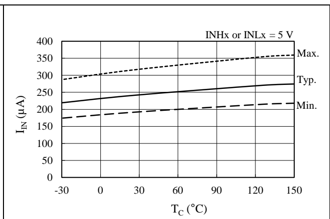
Figure 15-13. Input Current at High Level ( I_{IN} or I_{INx} ), I_{IN} vs. T_C
