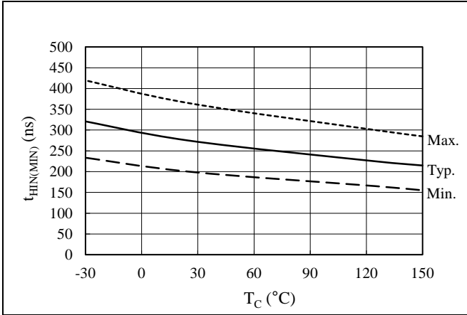
Figure 15-20. Minimum Transmittable Pulse Width for High-side Switching, t_{HIN(MIN)} vs. T_C
