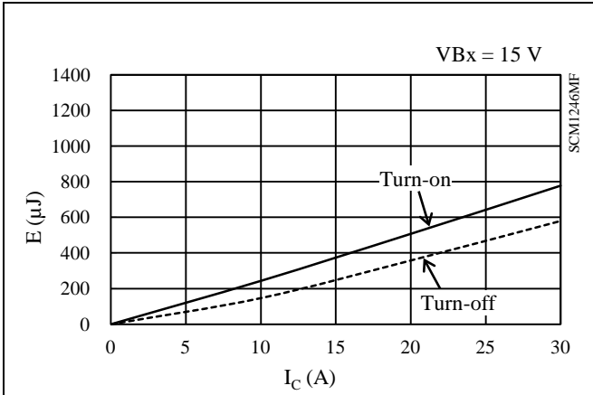
Figure 15-64. High-side Switching Loss (T j = 25 °C)
