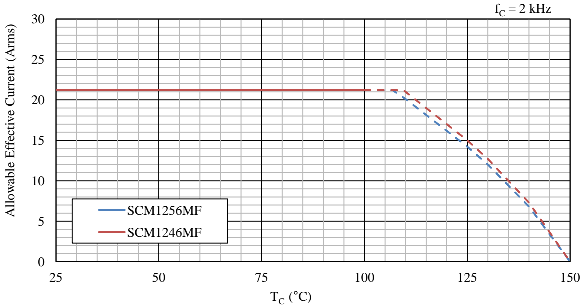
Figure 15-74. Allowable Effective Current, 30 A Device ( f_c = 2 kHz)
